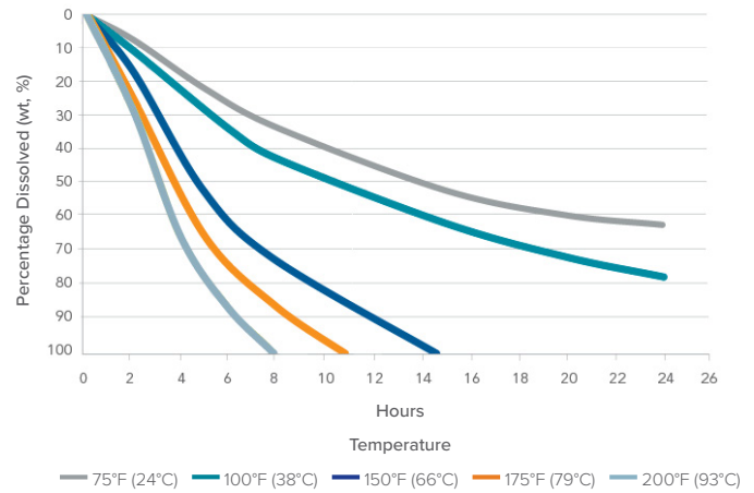
Solubility Profile 7/8" (22mm) in 15% Aqueous HCl
