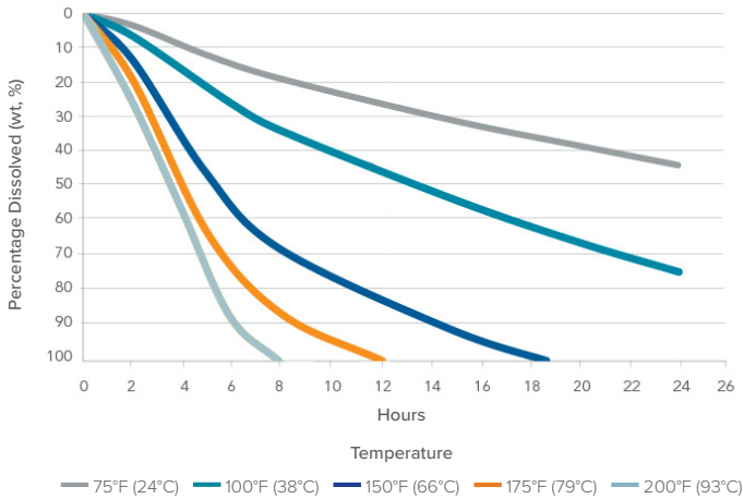
Solubility Profile 7/8" (22mm) in Aqueous NaOH (pH=11)
